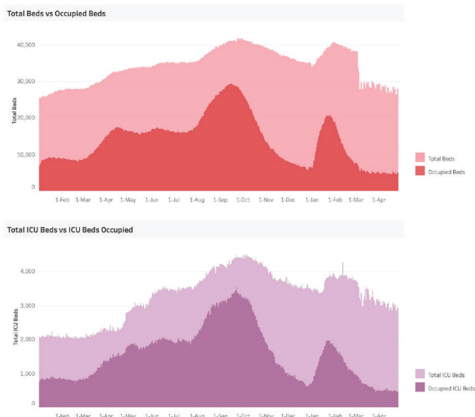
Figure 2. Total bed and ICU bed distribution over time stratified by occupancy (as of 8 May 2022)
