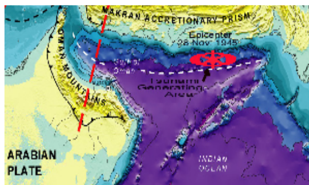
Figure 2.28 Location of Tsunami in 1945
